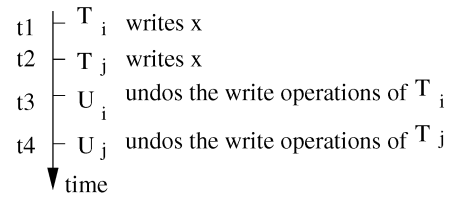
Fig. 9. Flaw of the straightforward undo method.
