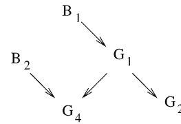
Fig. 3. Dependency graph for history H_3 .
