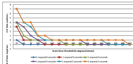
Fig. 6. False positives and negatives of shadow indicator checking for brute-force attack
